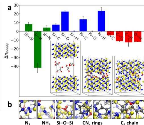
Figure 1: Superlow friction of \text{Si}_3\text{N}_4 tribopairs.
