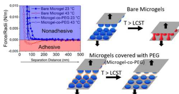
Scheme 1: Illustration of the Concept for Independent Control of Swelling and Surface Properties Using Thermo-Responsive PNIPAM Microgels Surface-Functionalized with (A) pH-Insensitive PEG and (B) pH-Sensitive PDMAEMA.
